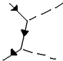
positron photon scattering
