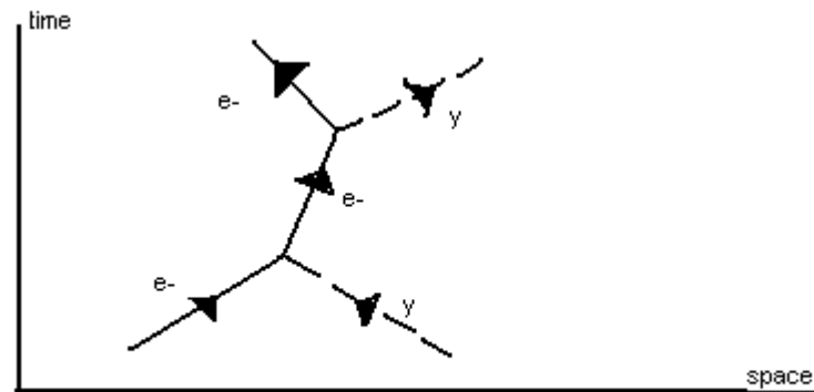
electron photon scattering
