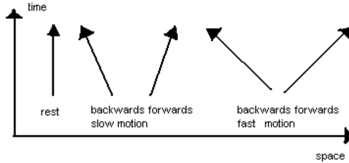
world lines of particles
