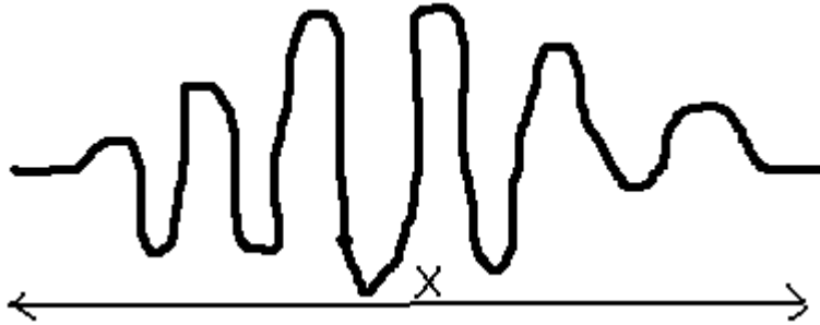
a wave packet corresponding to a particle located somewhere in the region X
